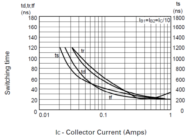
Switching Speeds
